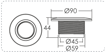
Suction Fitting
