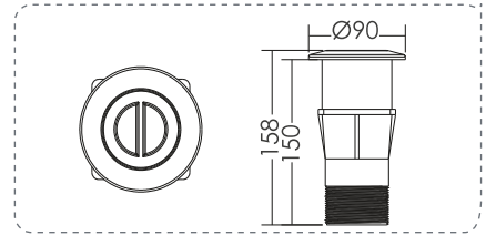
Vacuum Fitting (Concrete Pool)
