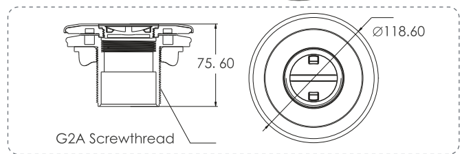
Vacuum Fitting (Vinyl Pool) EM2836
