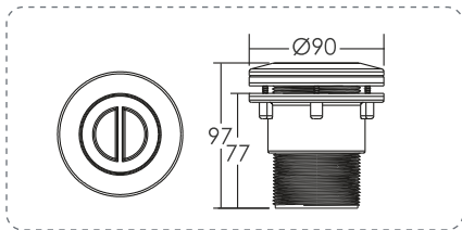
Vacuum Fitting (Vinyl Pool)
