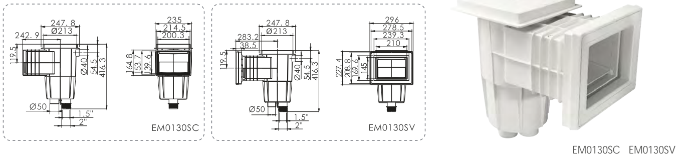
EM0130SC EM0130SV
