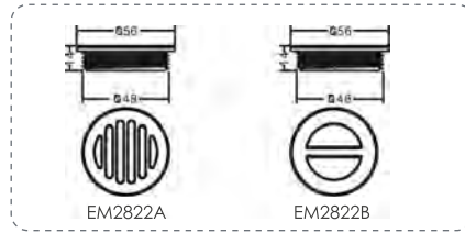
Cover of Suction Fittings
