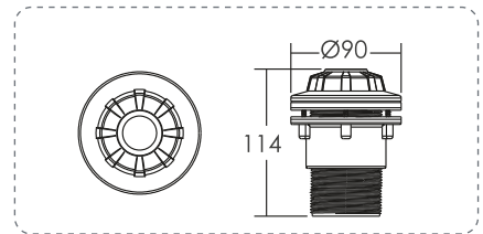
Outlet Fitting (Vinyl Pool)
