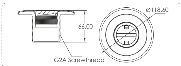
Vacuum Fitting (Concrete Pool) EM2831
