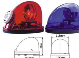
Halogen Rotator Beacon LTD508
