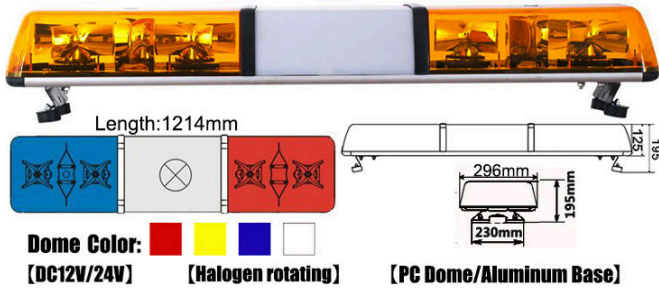
Halogen Rotator Vehicle Warning Lightbar TBD5015
