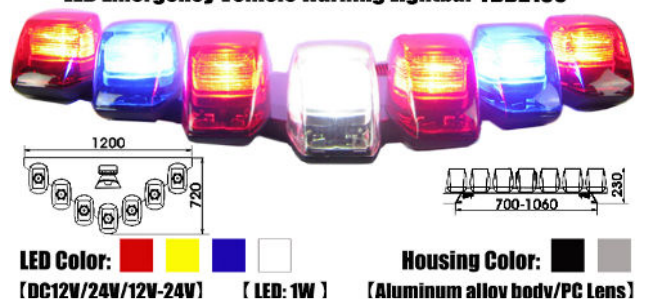
LED Emergency Vehicle warning Lightbar TBD2136
