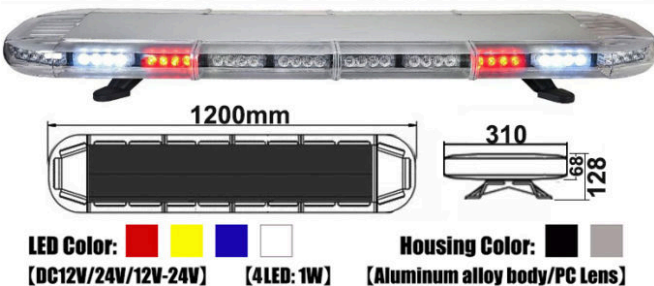
LED Emergency Vehicle warning Lightbar TBD2132
