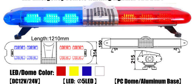
LED Emergency Vehicle warning Lightbar TBD2124
