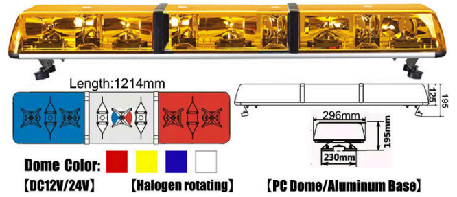
Halogen Rotator Vehicle Warning Lightbar TBD5015A
