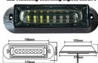
LED Flashing Warning Lights LED275
