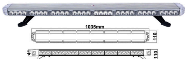
LED Emergency Vehicle warning Lightbar TBD2141
