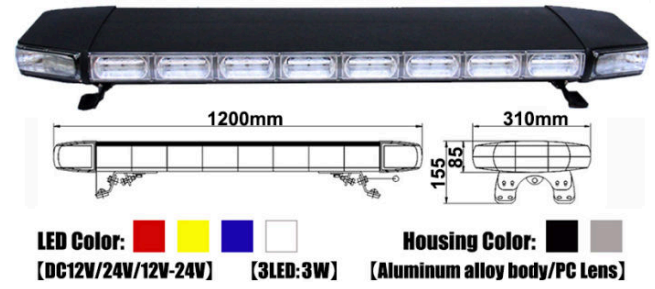
LED Emergency Vehicle warning Lightbar TBD2167
