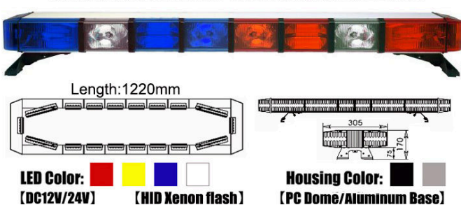
HID Xenon flash Vehicle Warning Lightbar TBD9001
