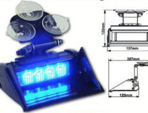
LED Visor Windshield Light: LED261D
