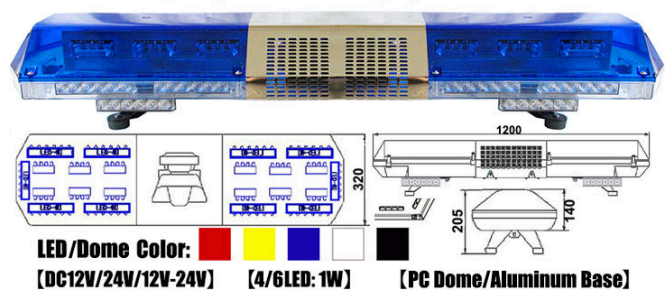
LED Emergency Vehicle warning Lightbar TBD5018L
