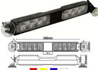
LED Visor Windshield Light: LED286
