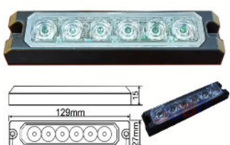
LED Flashing Warning Lights LED206B
