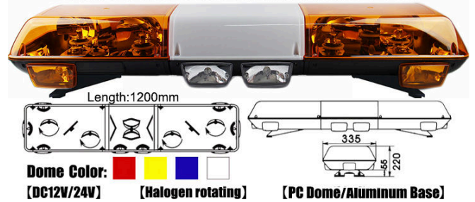
Halogen Rotator Vehicle Warning Lightbar TBD5014
