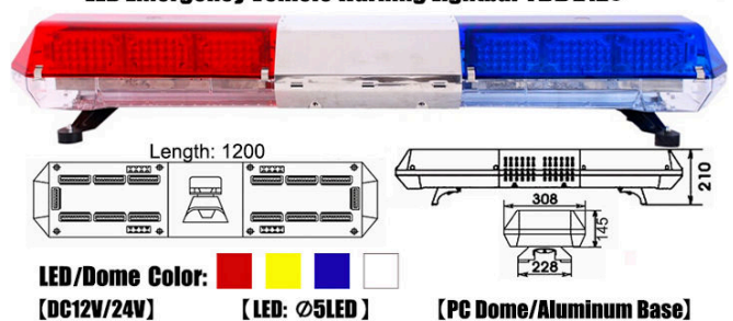
LED Emergency Vehicle warning Lightbar TBD2120
