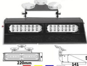
LED Visor Windshield Light: LED217
