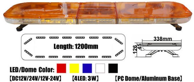
LED Emergency Vehicle warning Lightbar TBD2173
