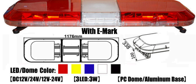
LED Emergency Vehicle warning Lightbar TBD2129
