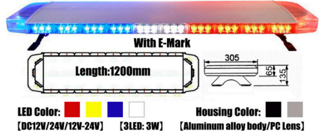
LED Emergency Vehicle warning Lightbar TBD2175
