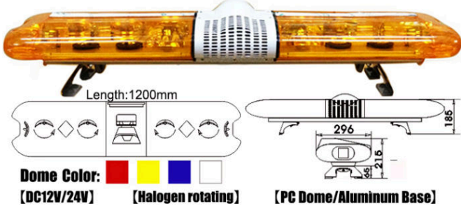
Halogen Rotator Vehicle Warning Lightbar TBD5011
