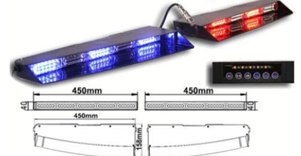
LED Visor Windshield Light: LED298
