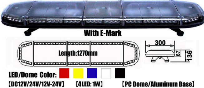
LED Emergency Vehicle warning Lightbar TBD2130
