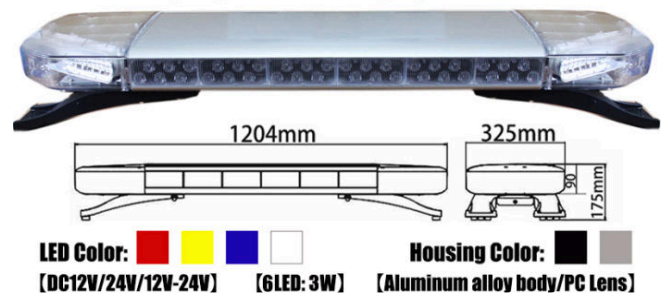
LED Emergency Vehicle warning Lightbar TBD2168
