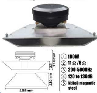
Loud Speaker YL-117
