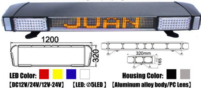
LED Vehicle Warning Display Lightbar TBD2125
