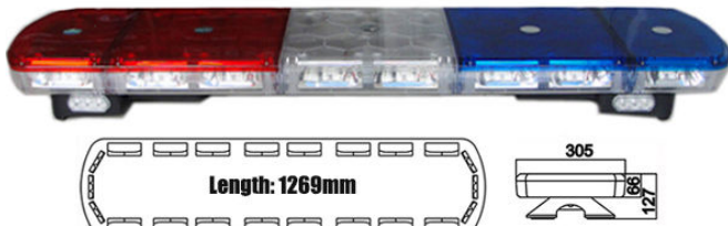
LED Emergency Vehicle warning Lightbar TBD2166
