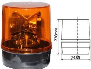
Halogen Rotator Beacon LTD504
