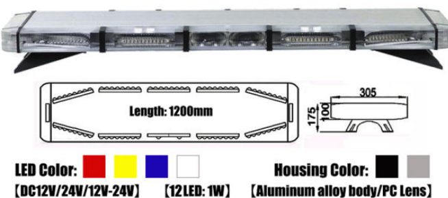
LED Emergency Vehicle warning Lightbar TBD2169
