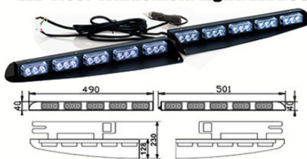
LED Visor Windshield Light: LED299
