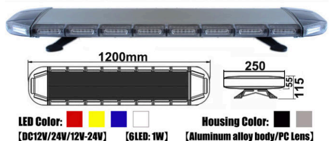
LED Emergency Vehicle warning Lightbar TBD2132B
