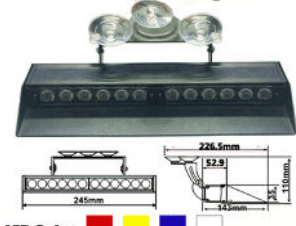
LED Visor Windshield Light: LED291D
