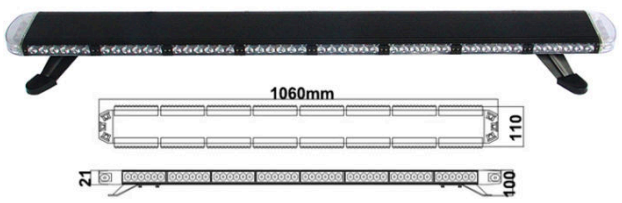
LED Emergency Vehicle warning Lightbar TBD2141B
