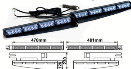
LED Visor Windshield Light: LED288
