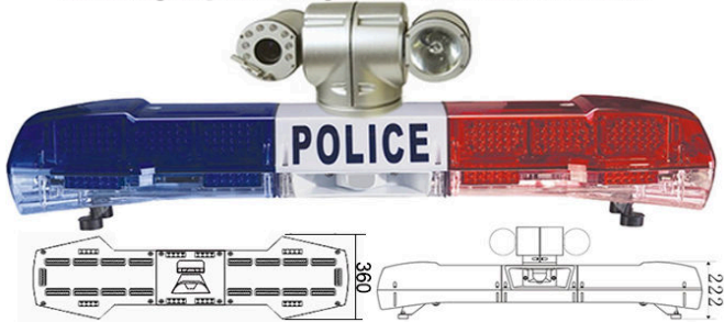
LED Emergency Vehicle Lightbar with Camera TBD2119CH
