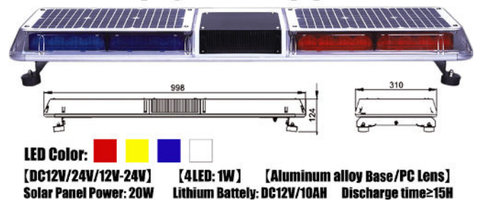
Solar LED Emergency Vehicle Warning Lightbar TBD3001KS
