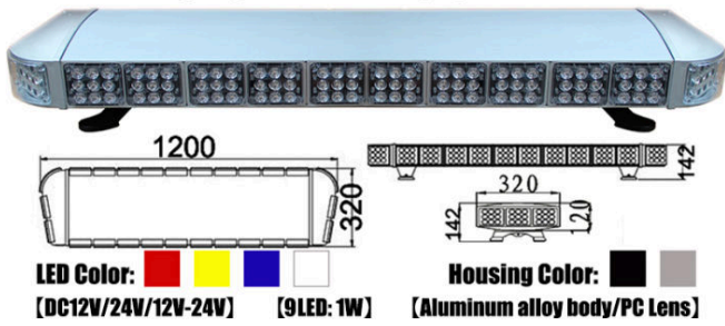
LED Emergency Vehicle warning Lightbar TBD2106
