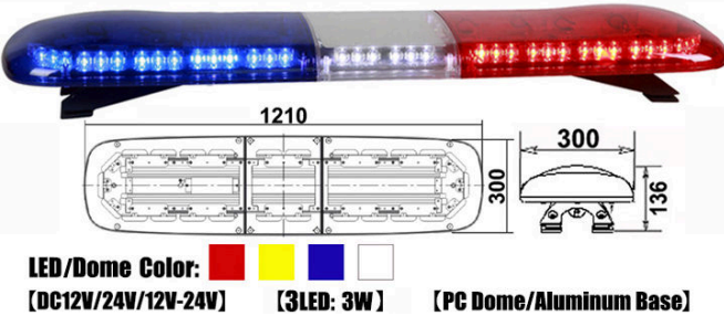
LED Emergency Vehicle warning Lightbar TBD2178
