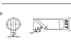
T800-K ACF028956
