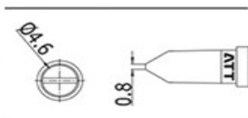
T800-4.6D ACF028955
