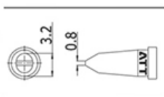
T800-3.2D ACF028954
