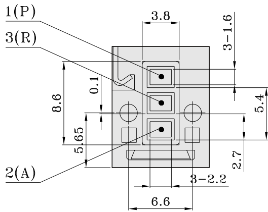
Installation Dimensions
