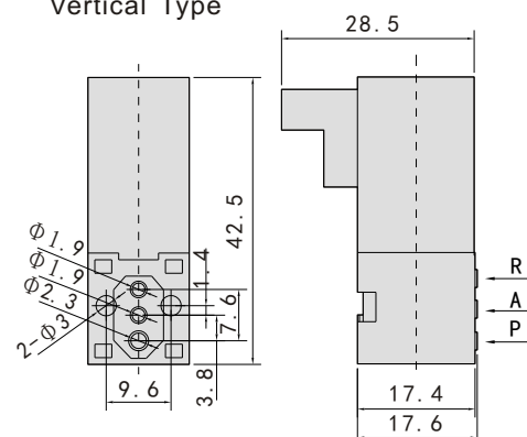
Vertical Type
