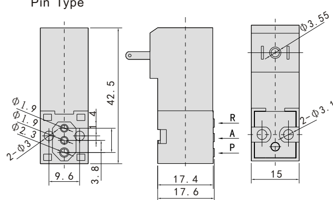
Pin Type
