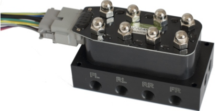
VU-4F G1/4" G3/8" NPT1/4" NPT3/8"
