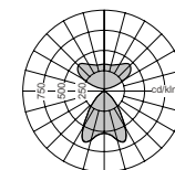
Indirect/direct light
