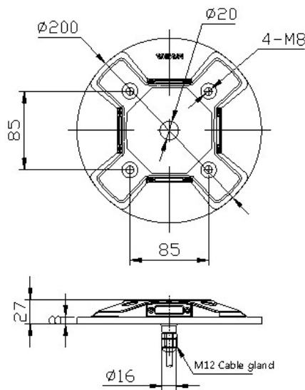
Dimension ( mm )
