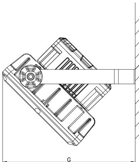
Wall Mount
