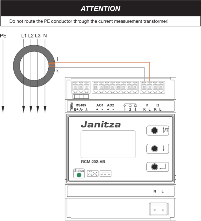
Fig. 3: Simplified presentation of residual current measurement
