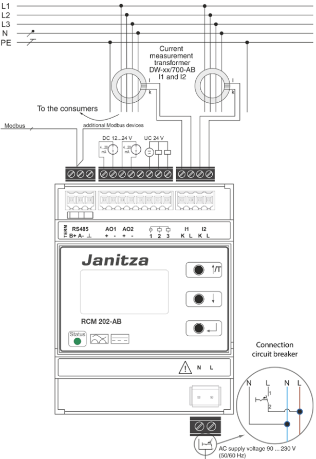
Fig. 4: Circuit diagram of the RCM 202-AB
