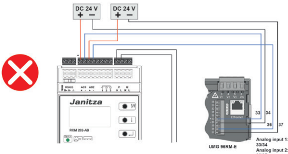
Fig. 8: Invalid connection scheme
