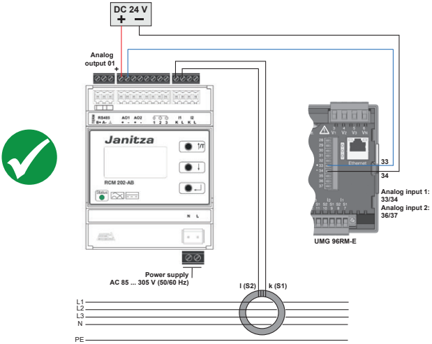
Fig. 7: Connection to the analogue inputs of a UMG 96RM-E
