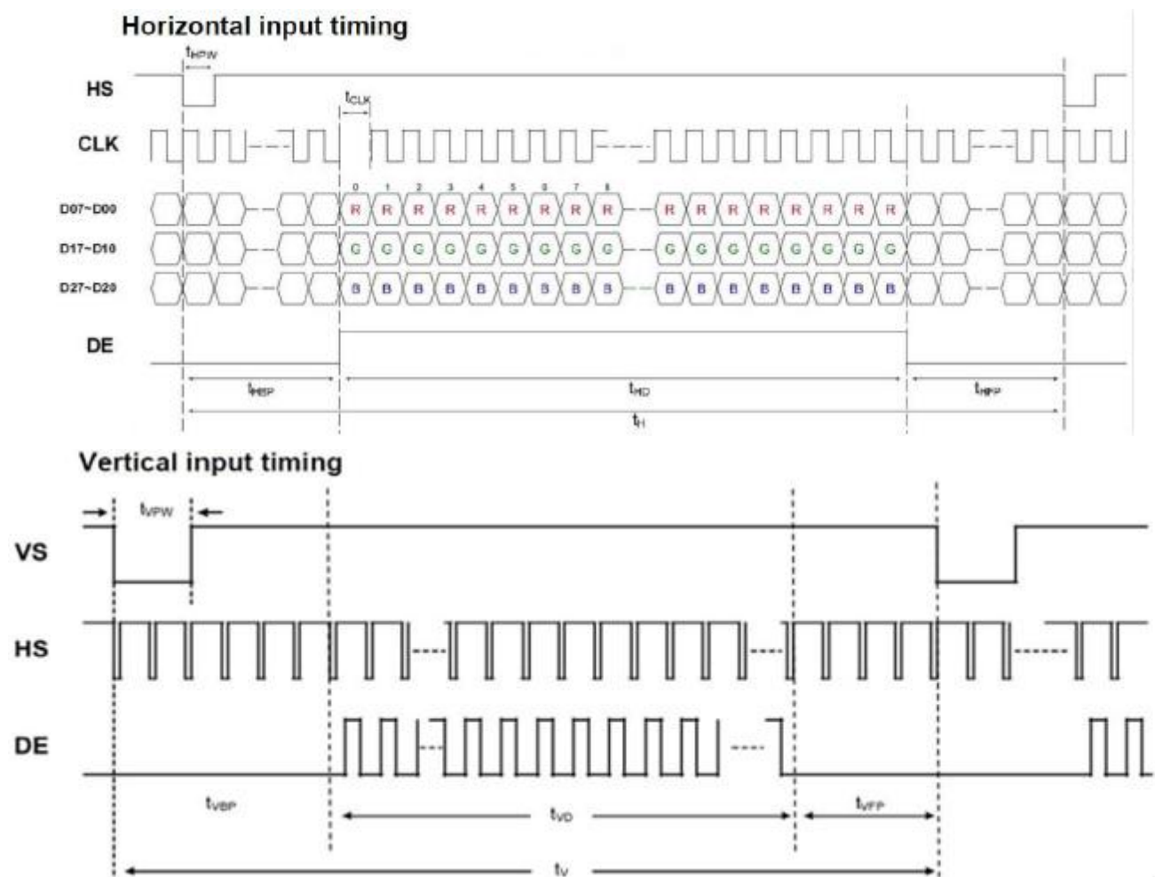
Figure 5.2 Input signal data timing
