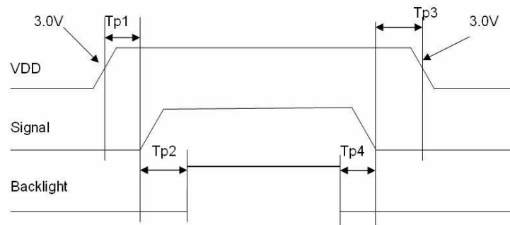
Interface Power On/Off Sequence
