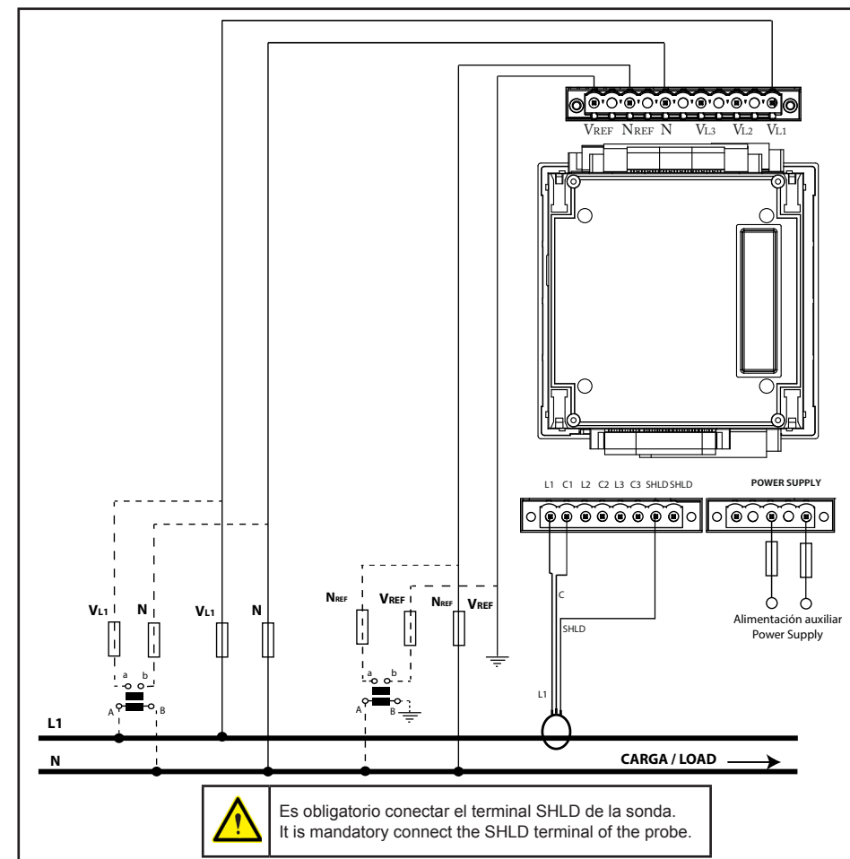
Red monofásica fase-neutro de 2 hilos / 2-wire Single-phase network (Neutral) Sonda FLEX-MAG .../100mV ~ / FLEX-MAG Probe .../100mV ~
