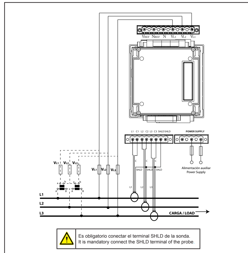
Red trifásica a 3 hilos / 3-wire three-phase network Transformadores de corriente .../5A o .../1A / .../5 or .../1A current transformers
