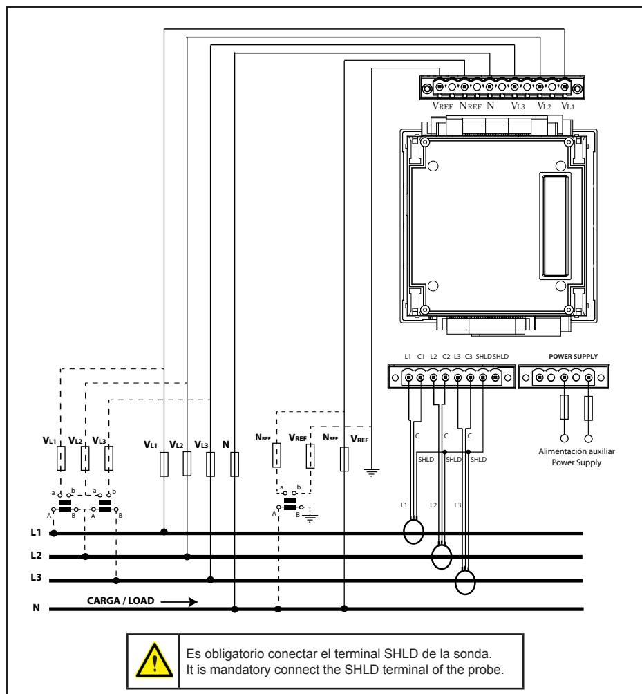
Red trifásica a 4 hilos / 4-wire three-phase network Sonda FLEX-MAG .../100mV ~ / FLEX-MAG Probe .../100mV ~
