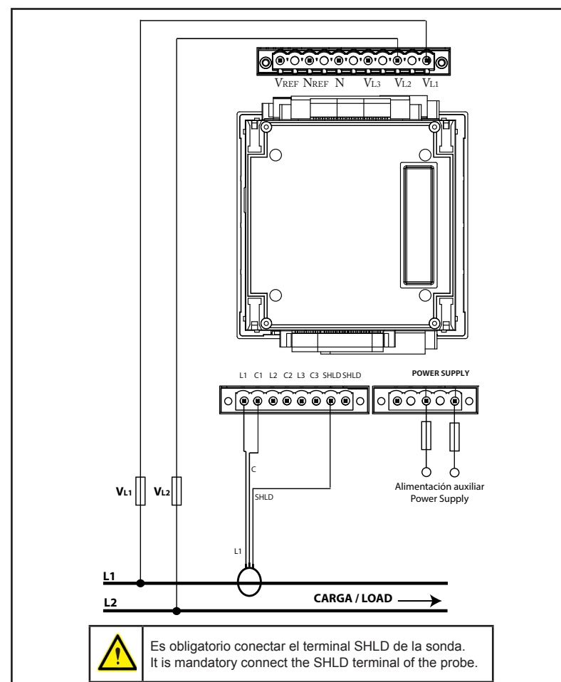
Red monofásica fase - fase de 2 hilos / 2-wire Single-phase network Phase - Phase Sonda FLEX-MAG .../100mV ~ / FLEX-MAG Probe .../100mV ~
