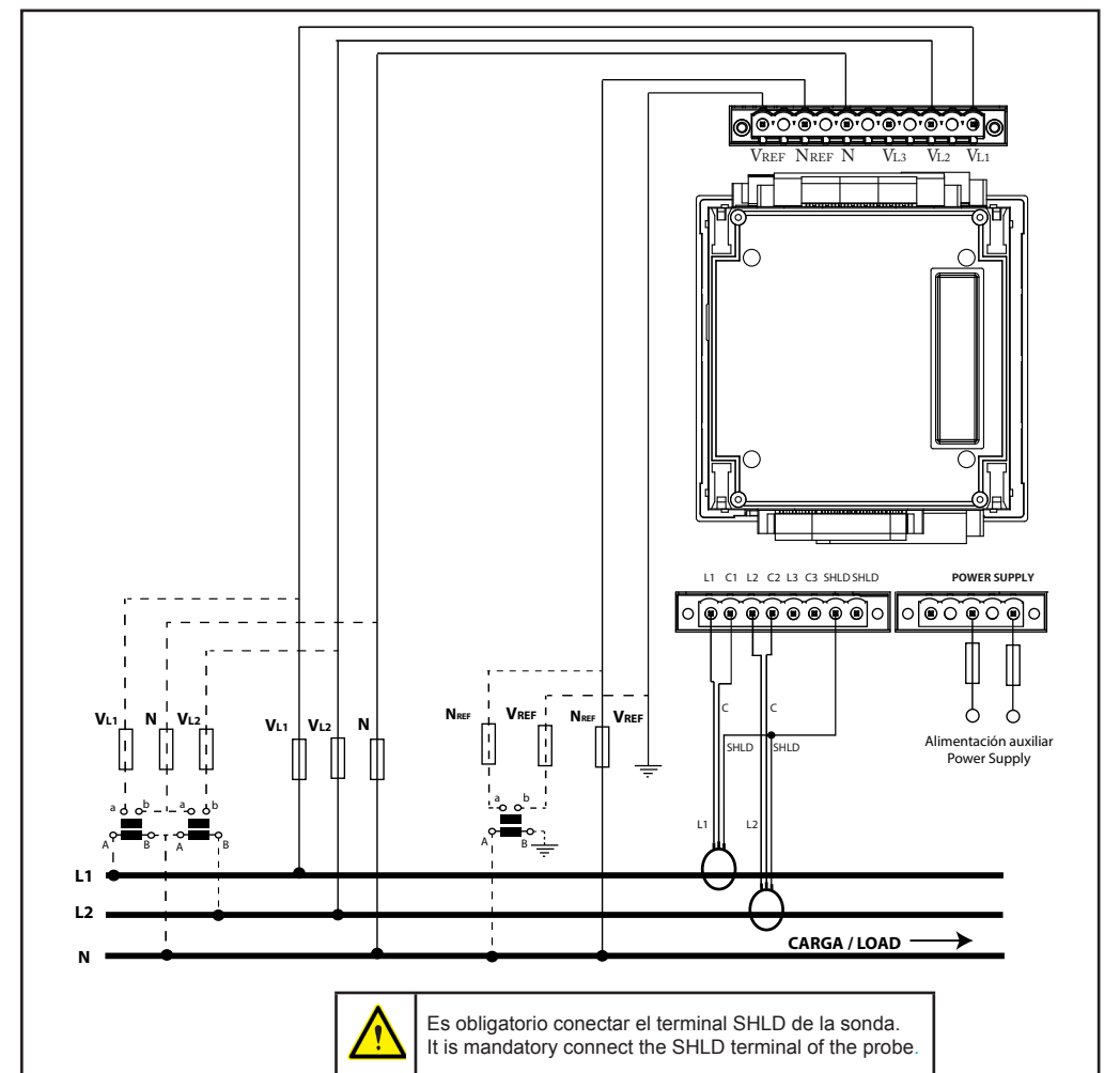
Red bifásica a 3 hilos / 3-wire two-phase network Transformadores de corriente .../5A o .../1A / .../5 or .../1A current transformers
