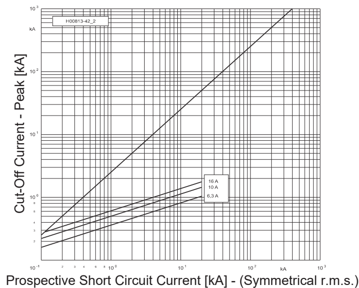
Cut-Off Current
