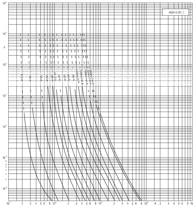
Minimum Melting
