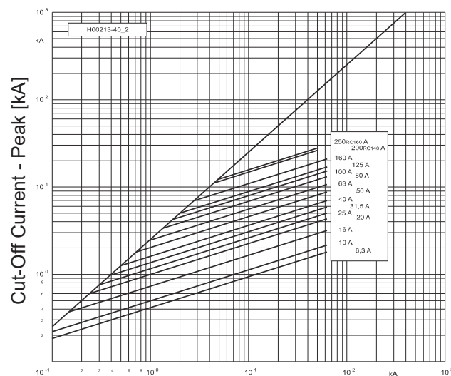
Cut-Off Current
