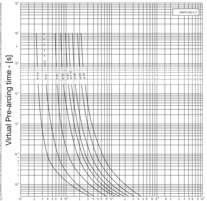
Total Clearing
