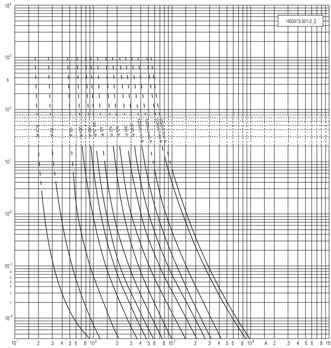
Minimum Melting
