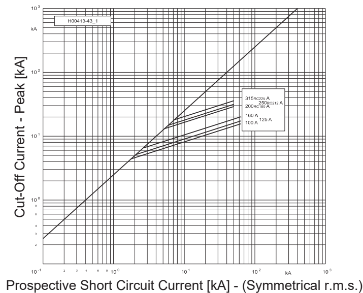
Cut-Off Current
