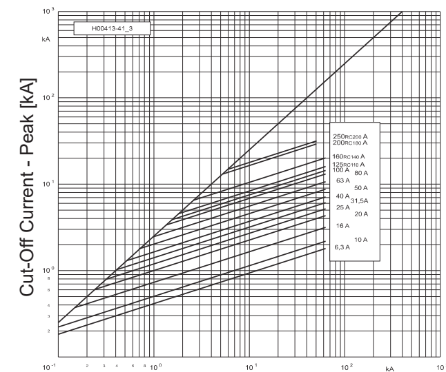
Cut-Off Current
