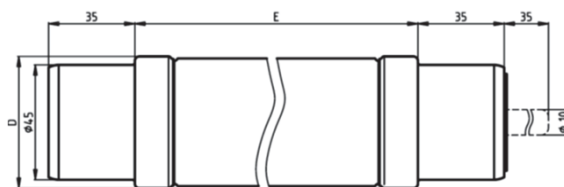
Dimensions [mm]
