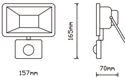
PS-FL-LED082SS-30W
