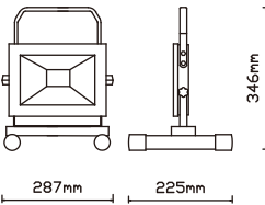
PS-FL-LED080-50W
