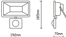
PS-FL-LED082SS-50W
