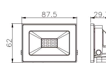
PS-FL-LED081-10W
