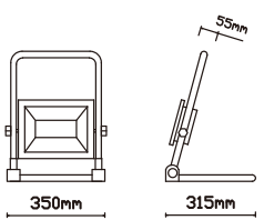
PS-FL-LED072-50W
