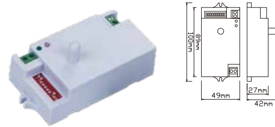
PS-RS34D
