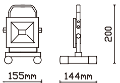
PS-FL-LED074-20W
