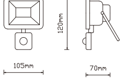
PS-FL-LED082SS-10W
