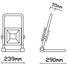
PS-FL-LED072-30W
