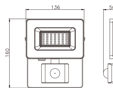
PS-FL-LED081SS-30W
