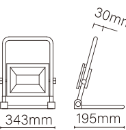
PS-FL-LED078-50W
