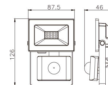
PS-FL-LED081SS-10W
