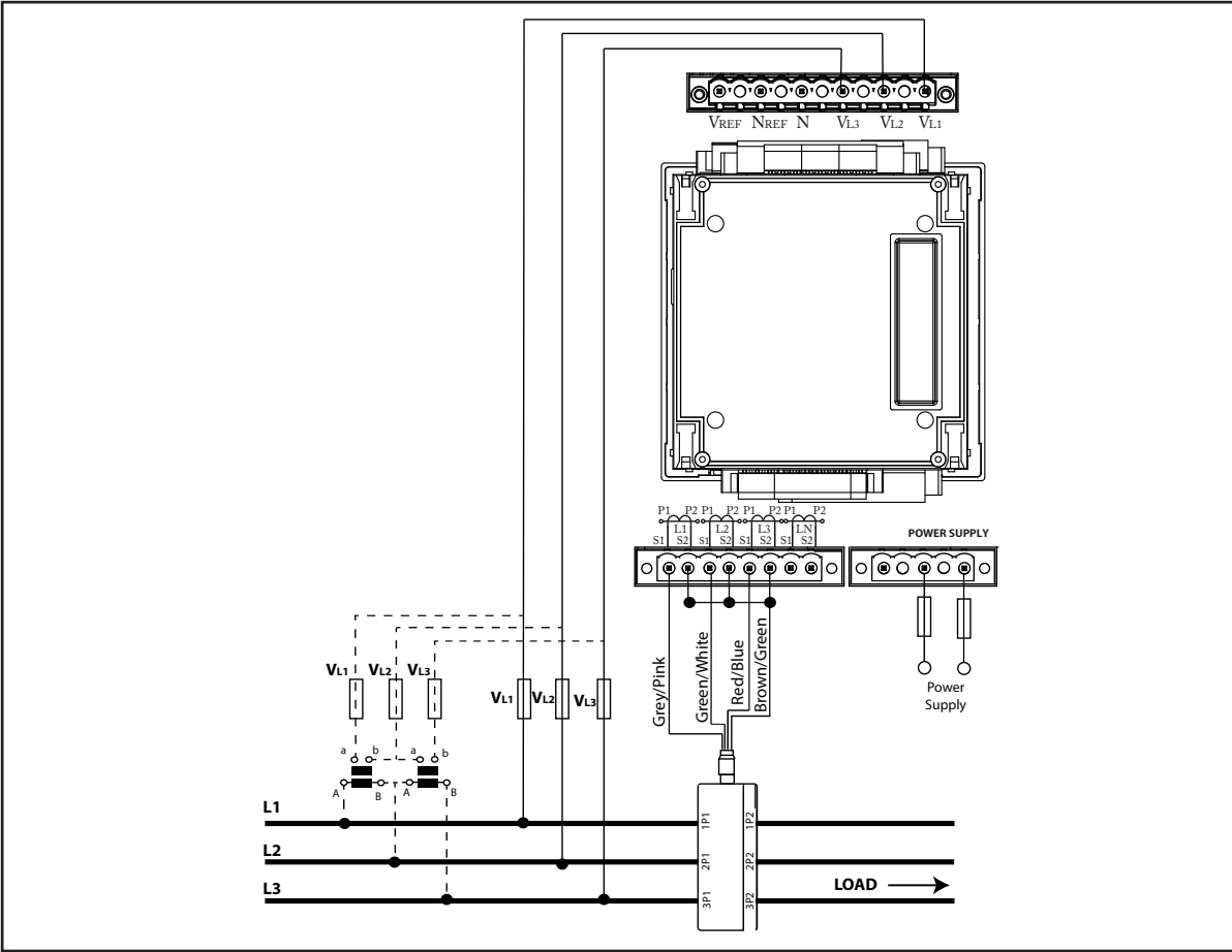
Red trifásica a 3 hilos / 3-wire three-phase network Transformadores de corriente serie MC3 (.../0.250 A) / MC3(.../0.250A) serial current transformers
