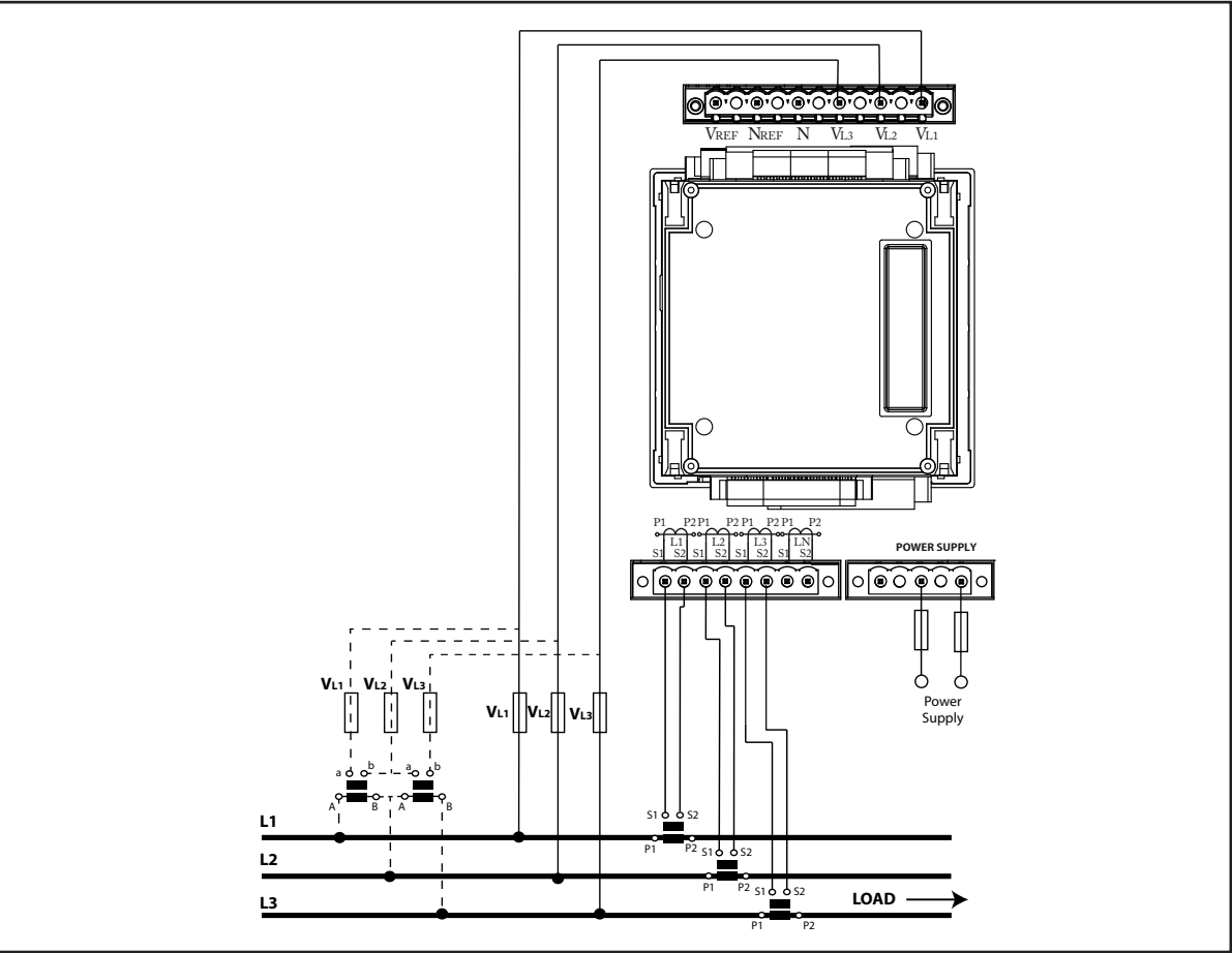
Red trifásica a 3 hilos / 3-wire three-phase network Transformadores de corriente .../5A o .../1A / .../5 or .../1A current transformers
