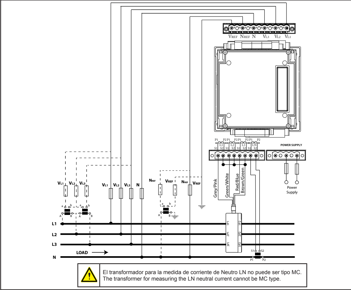
Red trifásica a 4 hilos / 4-wire three-phase network Transformadores de corriente serie MC3 (.../0.250 A) / MC3(.../0.250A) serial current transformers
