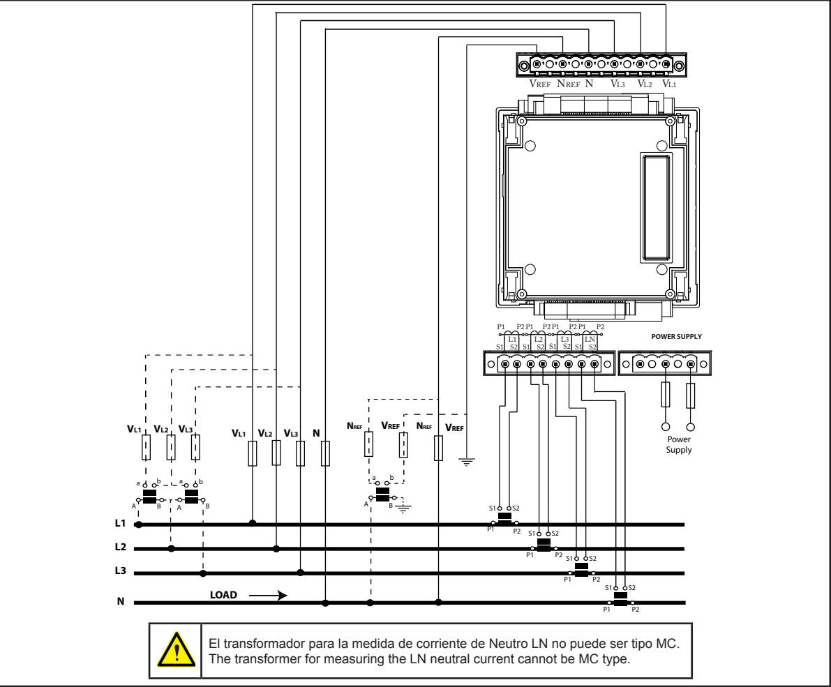
Red trifásica a 4 hilos / 4-wire three-phase network Transformadores de corriente .../5A o .../1A / .../5 or .../1A current transformers
