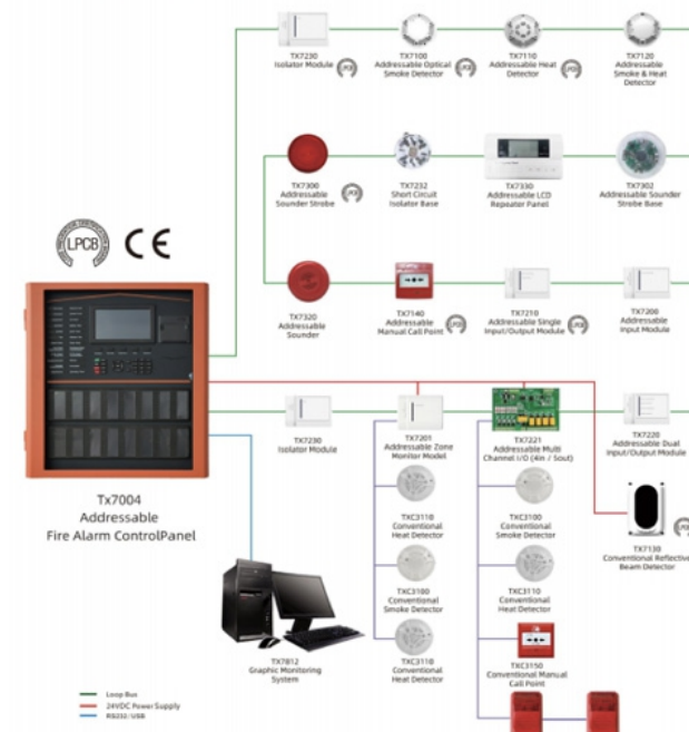
TX7 Intelligent Fire Alarm Control Panel (LPCB Approved)
