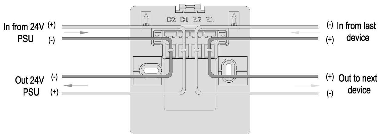
Figure 3: Wiring Details
