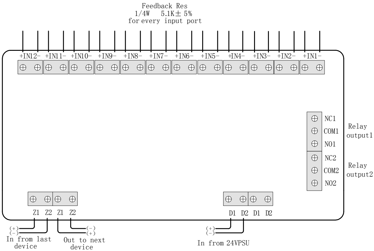
Figure 2 Wiring Details
