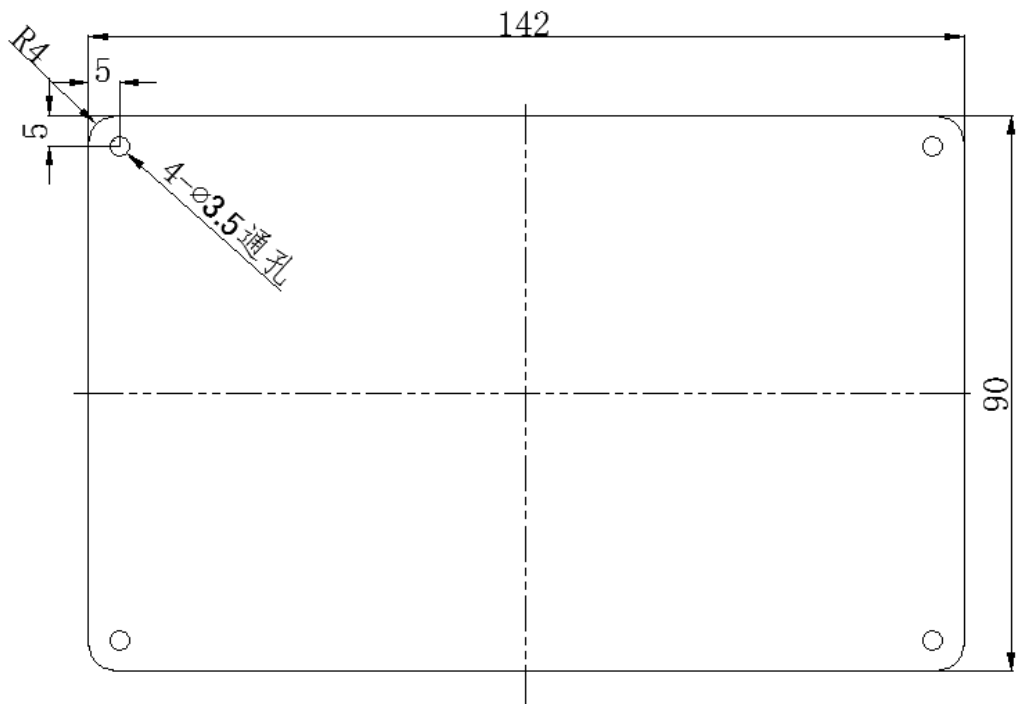
Figure 1 module outline diagram
