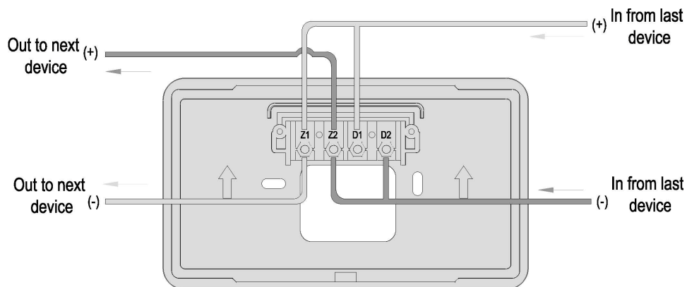
Figure 4 Loop Powered
