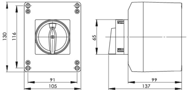
48x48 mounting enclosure : DS-ES1
