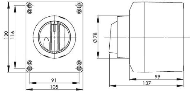
22Φ mounting enclosure : DS-ER1
