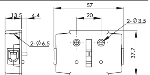
48x48 mounting enclosure : DS-ES2
