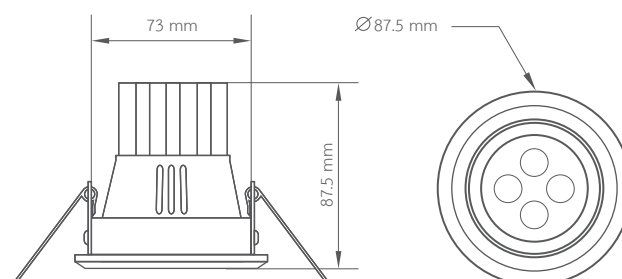
LFC-401D-3K0 / LFC-401A-3K0
