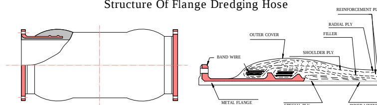
Structure Of Flange Dredging Hose
