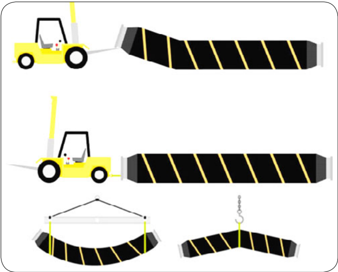
✗ Wrong ways to lift dredge hose
