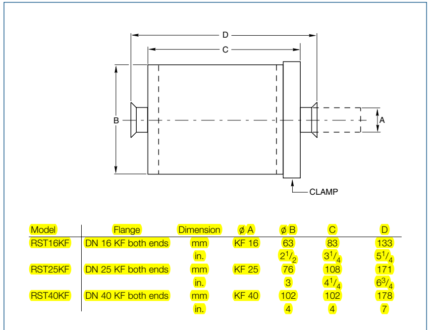
Dimensional drawing for the RST
