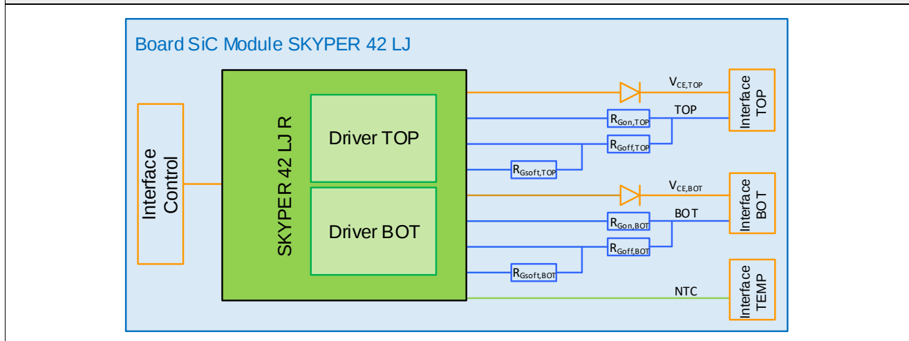
Figure 5: Board SiC Module SKYPER 42 LJ block diagram
