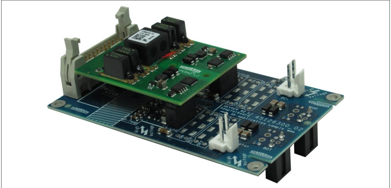
Figure 1: Board SiC Module SKYPER 42 LJ
