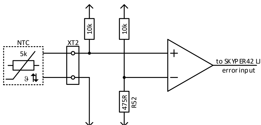
Figure 9: Schematic of NTC evaluation
