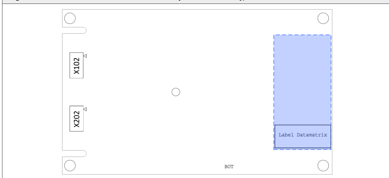
Figure 7: Board SiC Module SKYPER 42 LJ ("driver board"), bottom side
