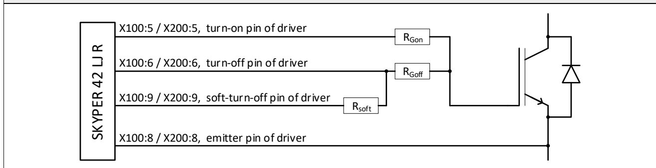
Figure 11: Schematic of gate resistor arrangement
