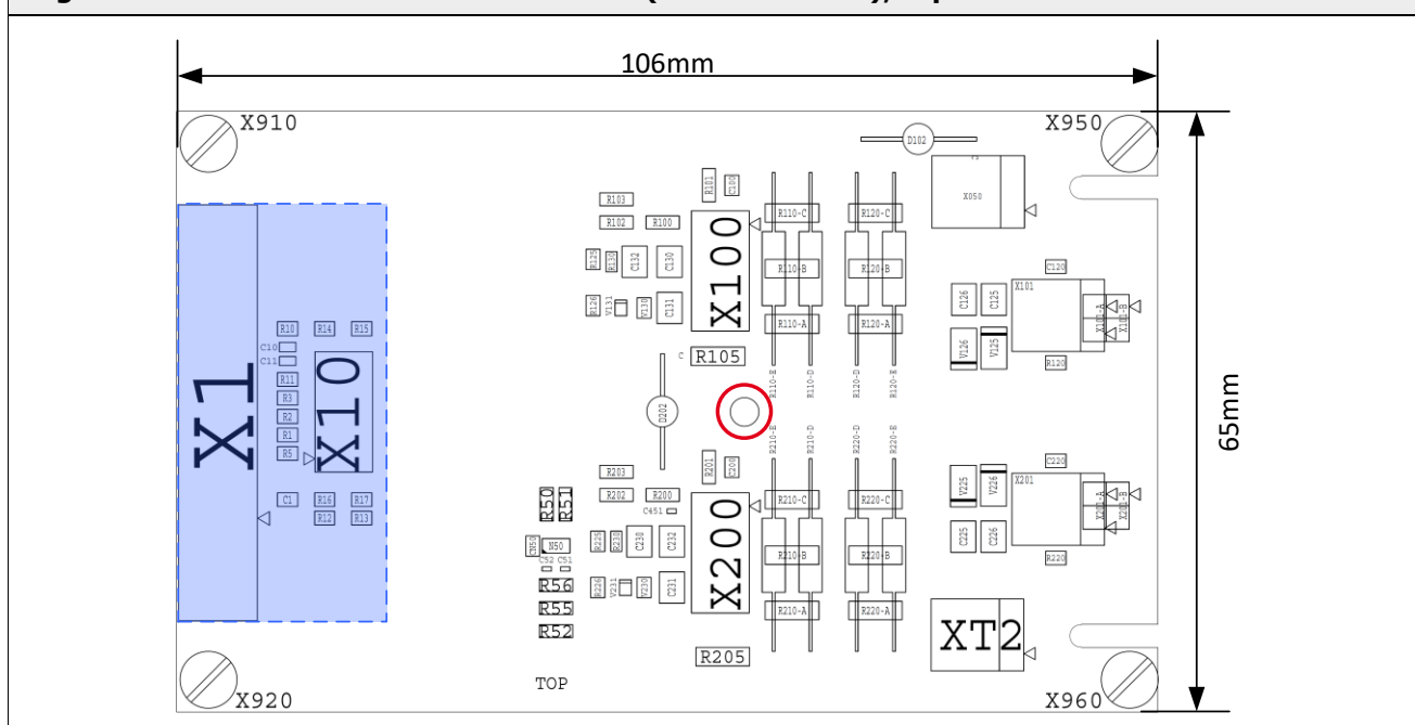
Figure 6: Board SiC Module SKYPER 42 LJ ("driver board"), top side
