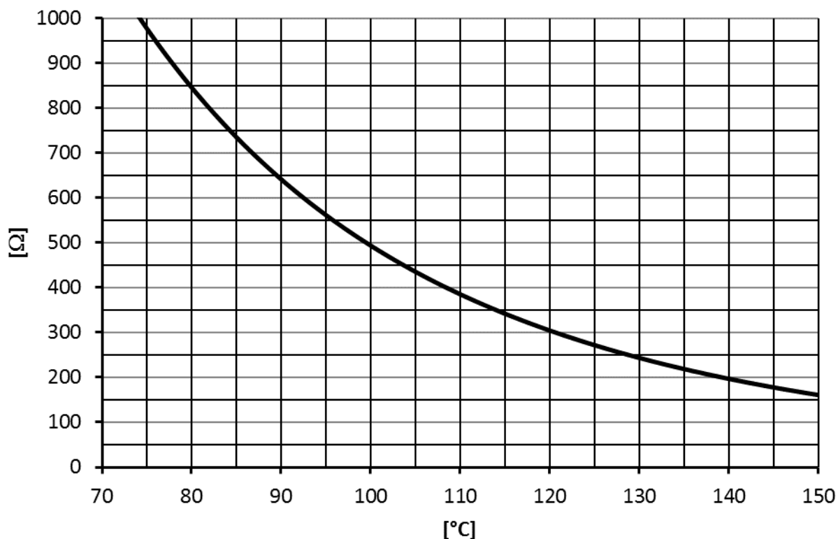
Figure 10: SEMIKRON NTC characteristic (excerpt)
