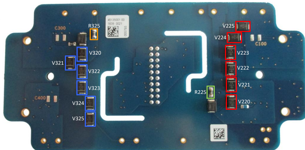
Figure 9: Bottom side of the driver board; user-changeable components are framed
