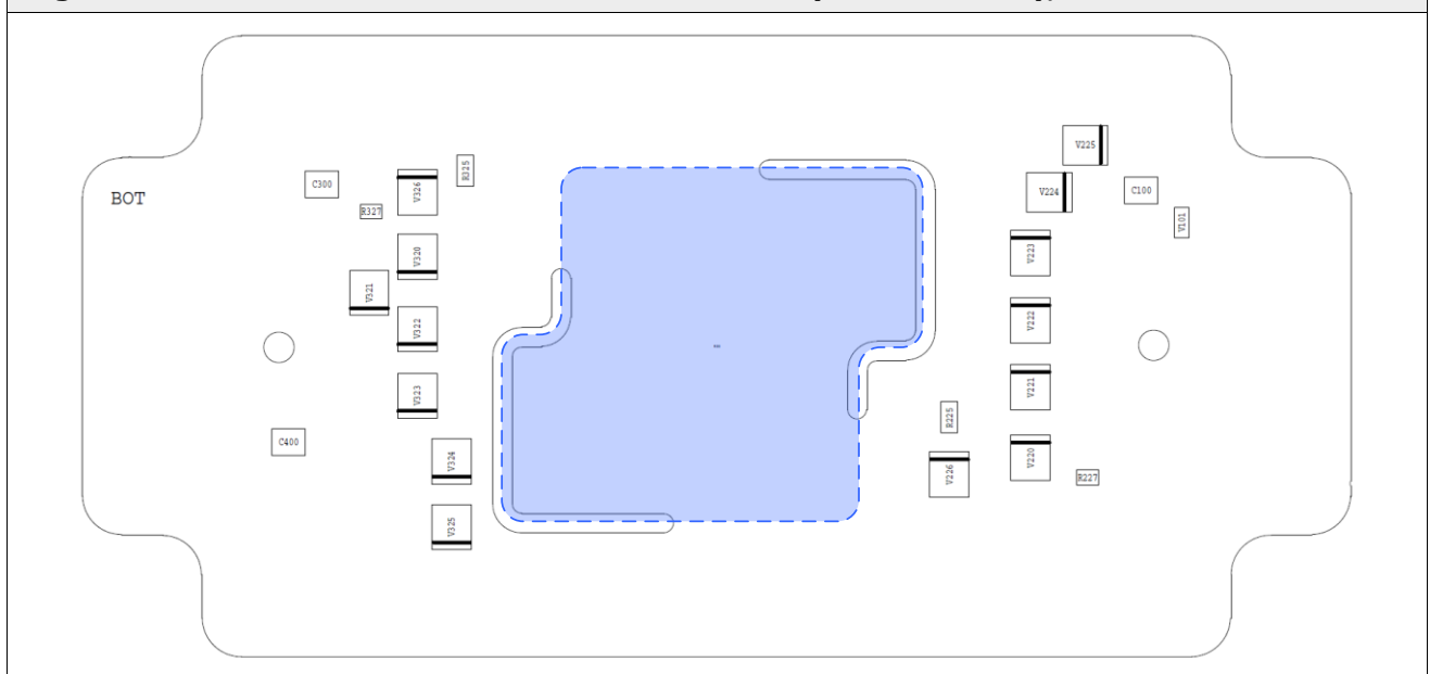
Figure 7: SEMiX5 1200V MLI SKYPER12 Driver Board ("driver board"), bottom side
