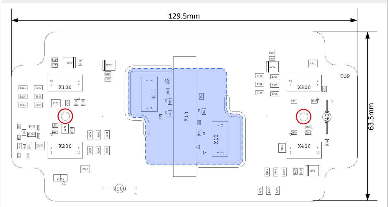
Figure 6: SEMiX5 1200V MLI SKYPER12 Driver Board ("driver board"), top side
