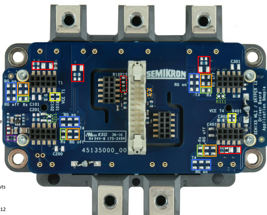
Figure 8: Top side of the driver board; user-changeable components are framed
