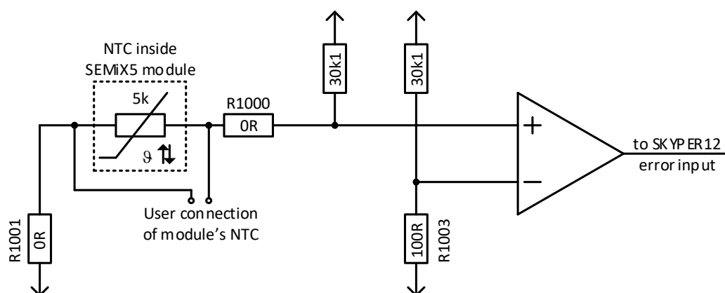
Figure 10: Schematic of NTC evaluation
