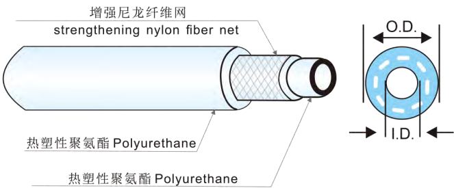
夹纱管结构图/Tube structure of the gripper
