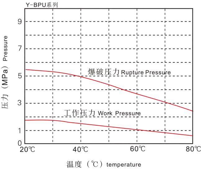
技术参数曲线图/ Technical parametersgraph
