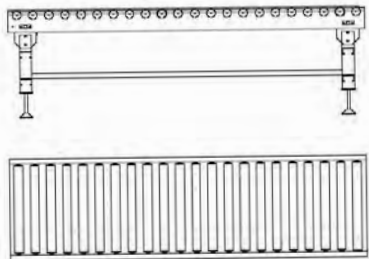
RC1M/2M 无动力滚筒输送台 Non-drive Roller Conveyor
