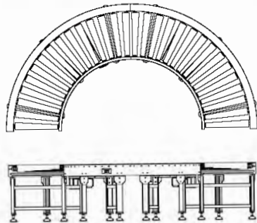
RCY180 动力滚筒圆角输送台 Corner Conveyor With Driving Force
