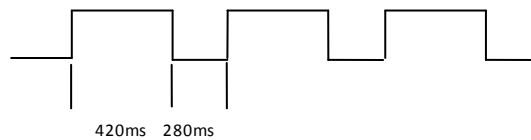
Fig.8 Fire alarm
