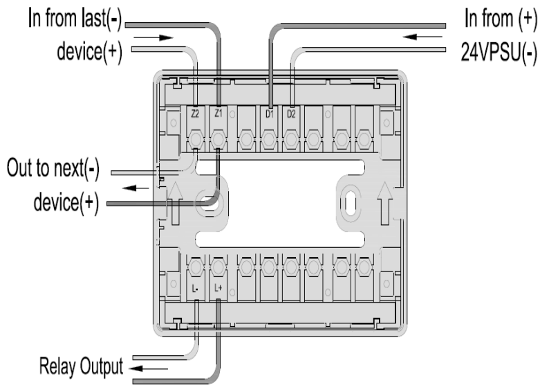
Figure 2: Wiring
